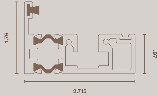
Upstand Track
