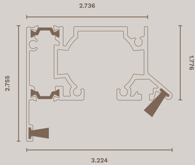
Coastal Storm Door Top Track
