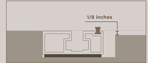
Flush track inset in subfloor
