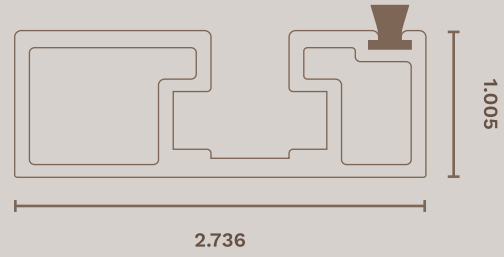
Flush Track
