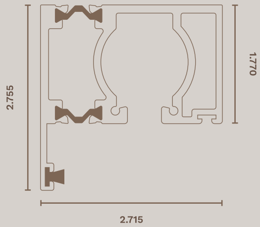
Top Track
