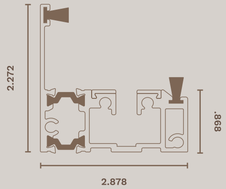
Coastal Storm Door Bottom Track
